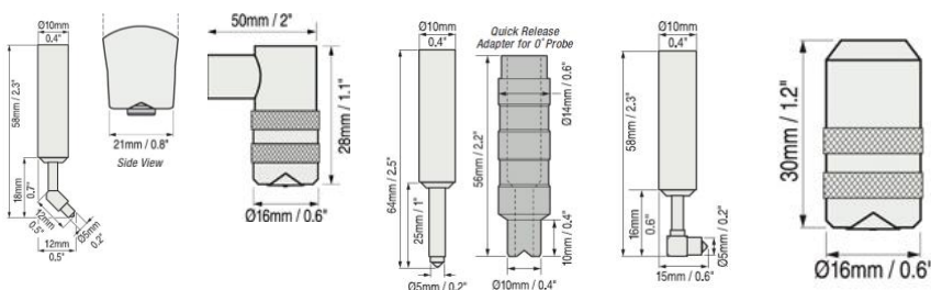
Fully Interchangeable Probes: Ferrous, non-ferrous, combination, thick, thin, etc. are compatible with ALL gage bodies.
